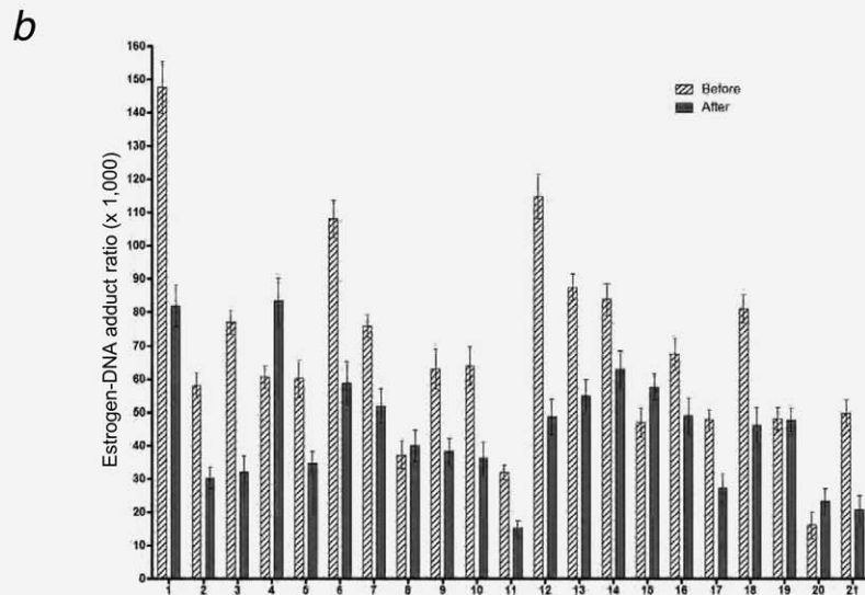
Figure 6. (a) Effects of NAC, Res, or NAC plus Res on the formation of depurinating estrogen-DNA adducts in MCF-10 F cells treated with 4-OHE 2 . The number above each bar indicates the percent inhibition compared to treatment with only 4-OHE 2 . 102 (b) Estrogen-DNA adduct ratios in women before and after following the Healthy Breast Protocol for three months. 103
