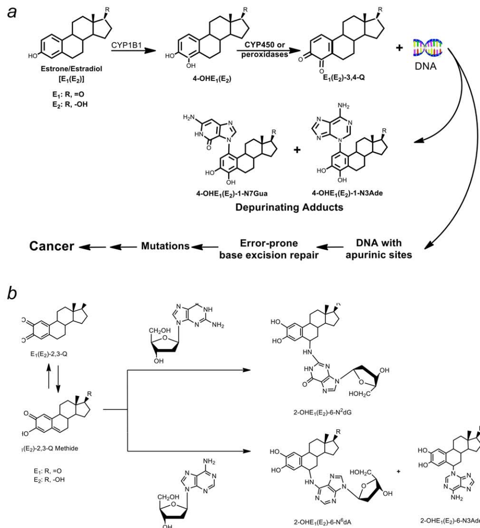
Figure 1. (a) Major metabolic pathway (97%) in cancer initiation. Reaction of E_1(E_2) -3,4-Q with DNA. (b) Reaction of E_1(E_2) -2,3-Q with dG or dA in DNA to form the two stable adducts 2-OHE _1(E_2) -6-N ^2 dG and 2-OHE _1(E_2) -6-N ^6 dA (<1%) and the depurinating adduct 2-OHE _1(E_2) -6-N3Ade (2%). [Color figure can be viewed at wileyonlinelibrary.com ]
